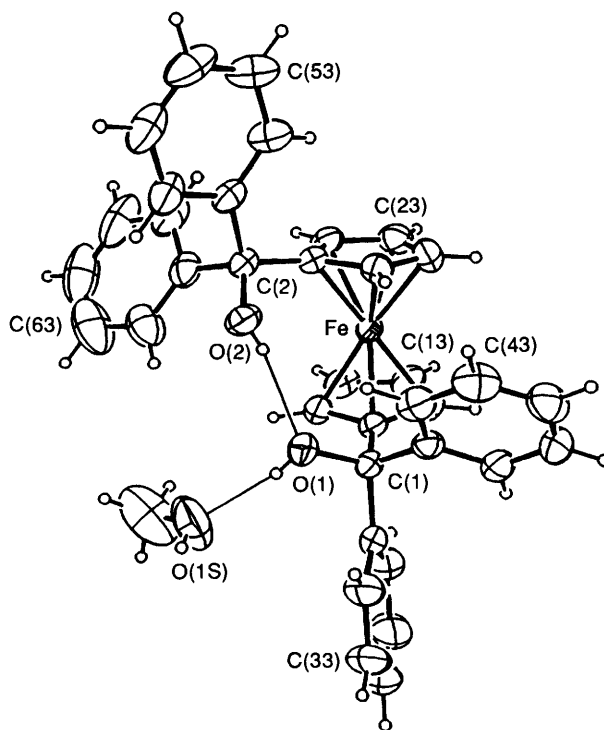
Fig. 1 A view of the asymmetric unit of the host-guest system 9a , [Fe(C 5 H 4 CPh 2 OH) 2 ] 2 ·MeOH, showing the atom-labelling scheme. For clarity the hydrogen atoms are drawn as small spheres of arbitrary size. All non-hydrogen atoms are depicted with their thermal ellipsoids at the 50% level
